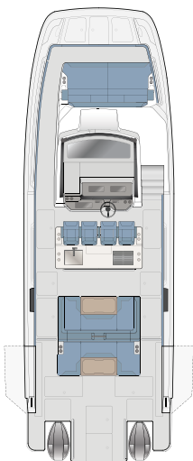
STANDARD MAIN DECK
