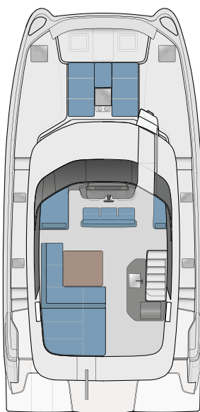
STANDARD FLYBRIDGE
